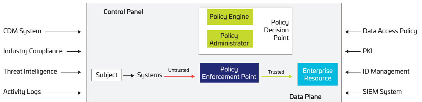
Figure 1: NIST Identity-Centric Zero Trust Architecture Approach. Source: NIST SP 800-207
