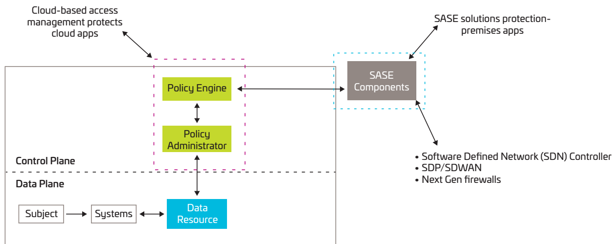
Figure 3: Combined, cloud based Zero Trust architecture approach.
