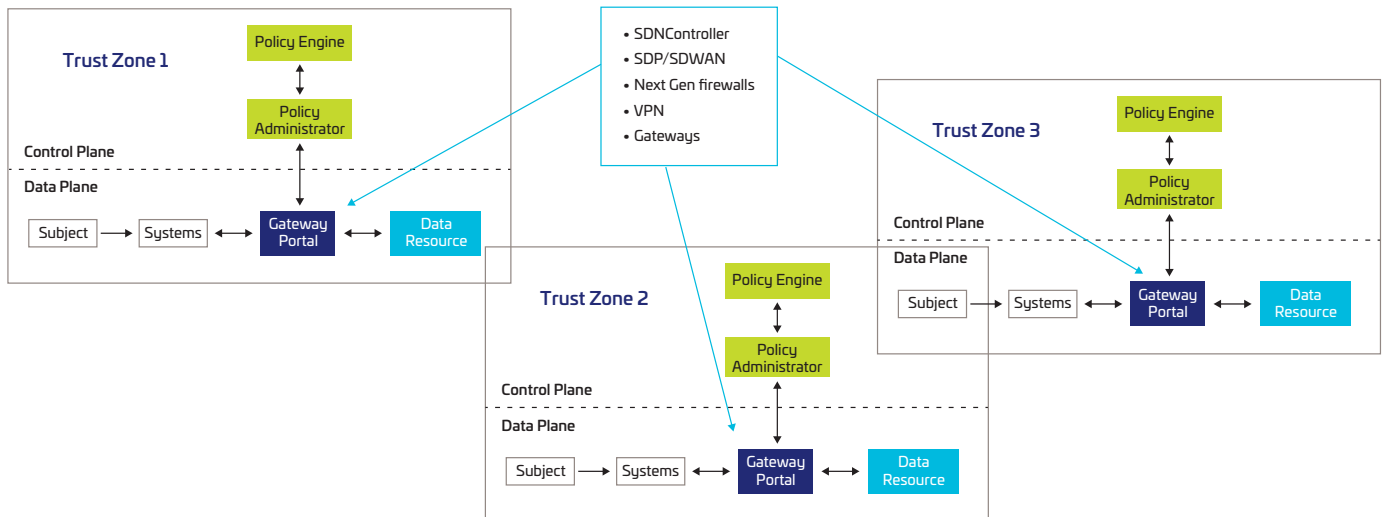
Figure 2: NIST Network-Centric Zero Trust Architecture Approach. Adapted from NIST SP 800-207.
